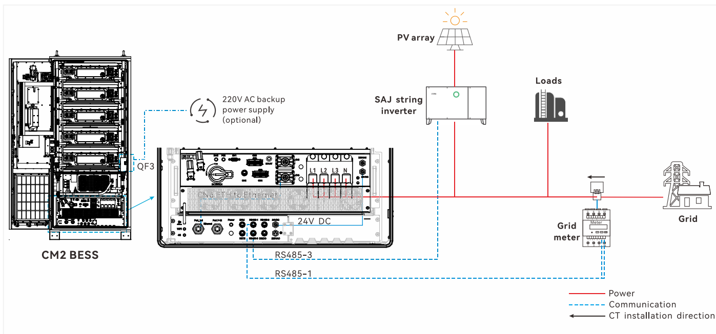
Figure 2.1. Single-cabinet connections
