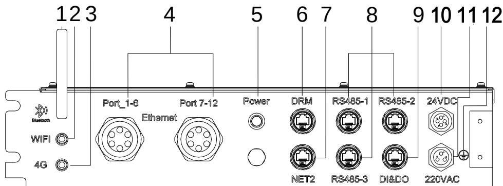
Figure 2.4. EMS unit electrical interfaces
